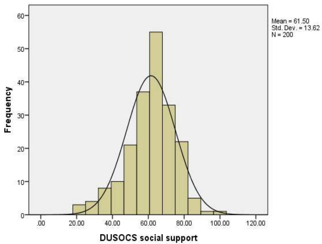
Figure G1. Histogram of DUSOCS social-support distribution.
