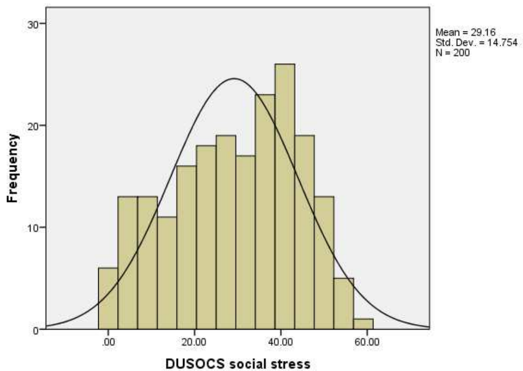
Figure G2. Histogram of DUSOCS social stress distribution.
