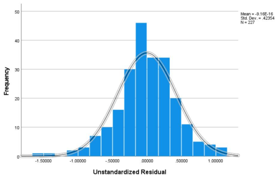
Histogram of Unstandardized Residuals
