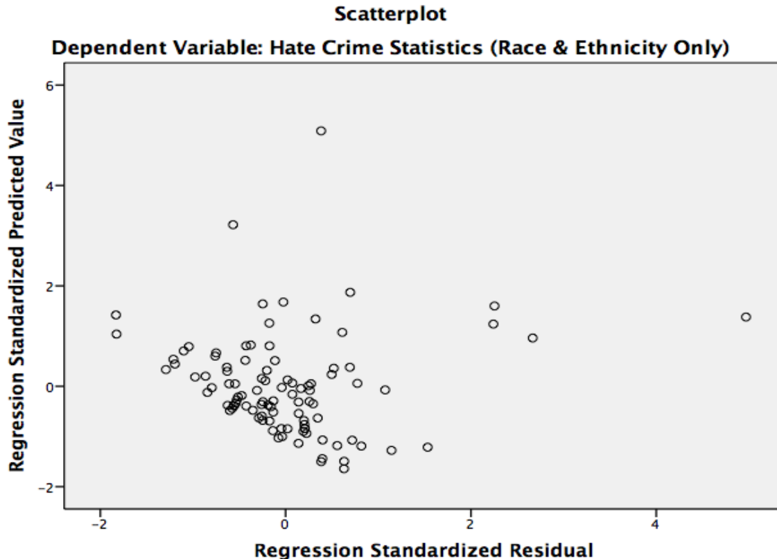
Figure 1. Plot of Standardized Residuals Versus Regression Standardized Predicted Value of Prediction of Hate Crime Rates by Different Demographic Diversity Rates
